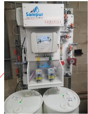
Monochloramine Generators
